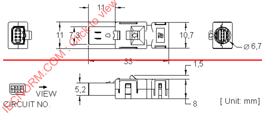
Figure B.2 – Dimensions of IMI cable connector
