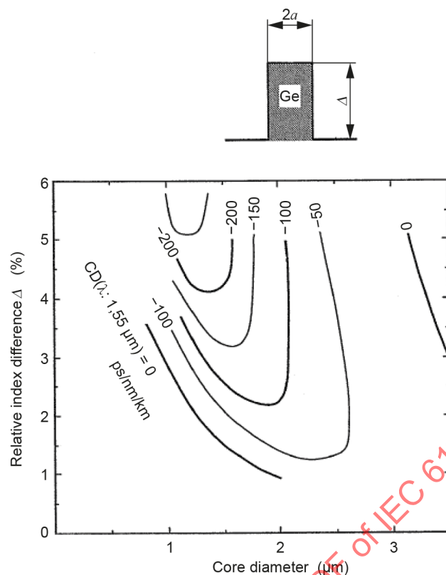
Figure A.2 – Calculated contour for different dispersion at the wavelength of 1,55 \mu\text{m} [ CD(\lambda: 1,55 \mu\text{m}) ] for a step index core fibre
