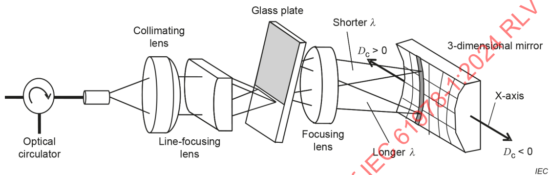
Figure C.1 – Structure of virtually imaged phased array (VIPA)
