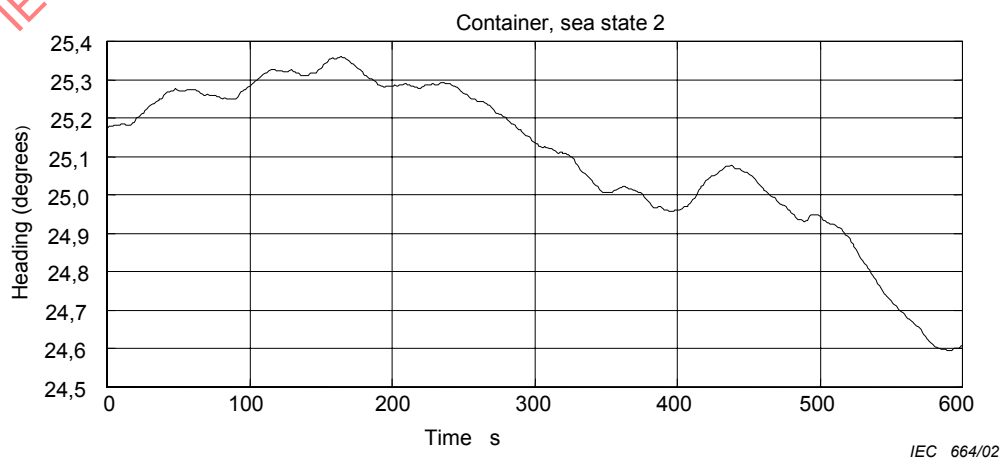
Figure H.7 – Container ship – sea state 2
