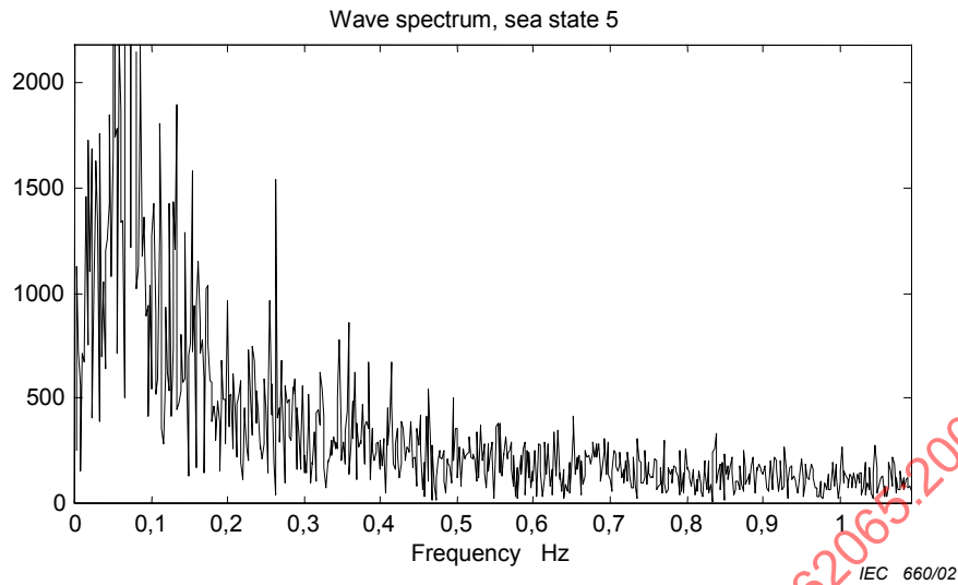
Figure H.3 – Wave spectrum – sea state 5
