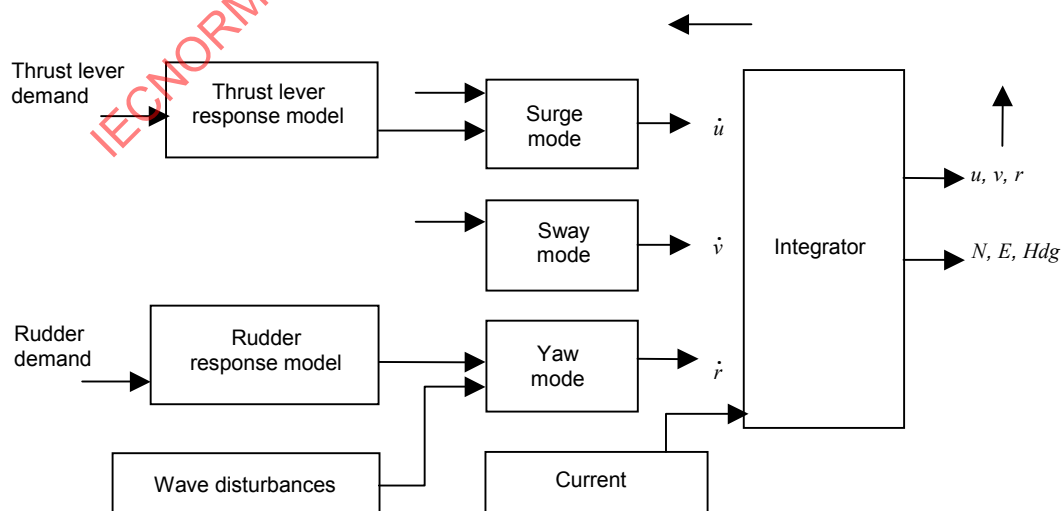
Figure I.1 – High level model block diagram
