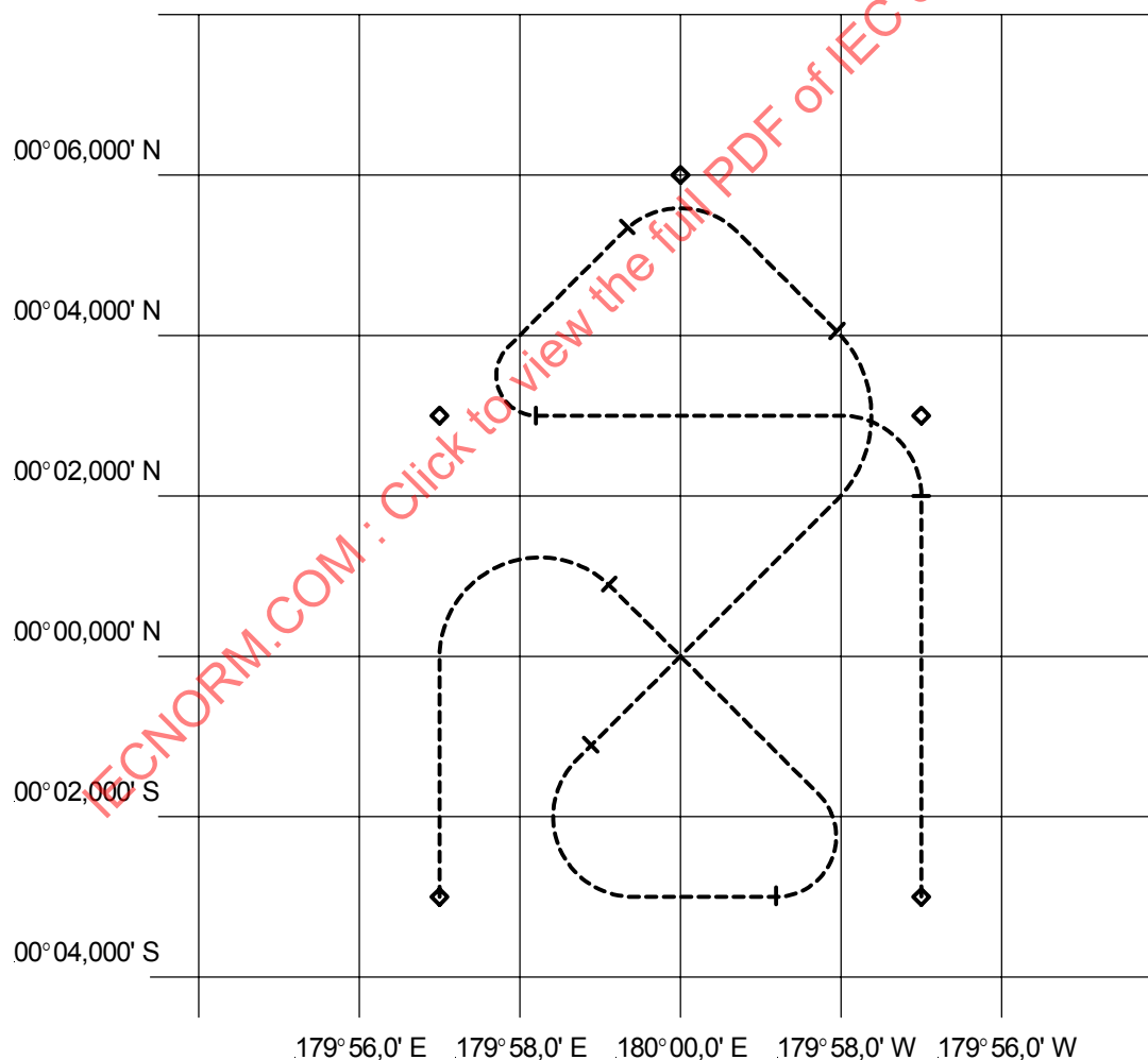
Figure G.2 – Scenario plot 2
