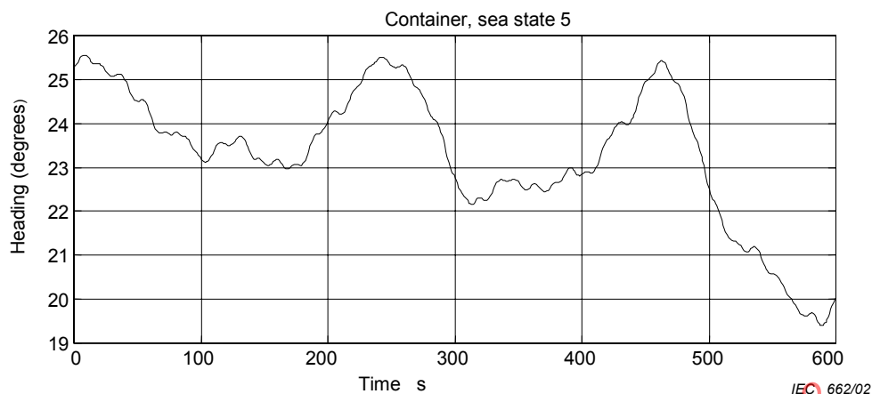
Figure H.5 – Container ship – sea state 5
