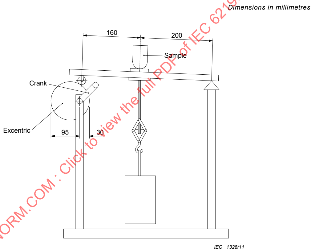
Figure 11 – Apparatus for testing the cable anchorage
