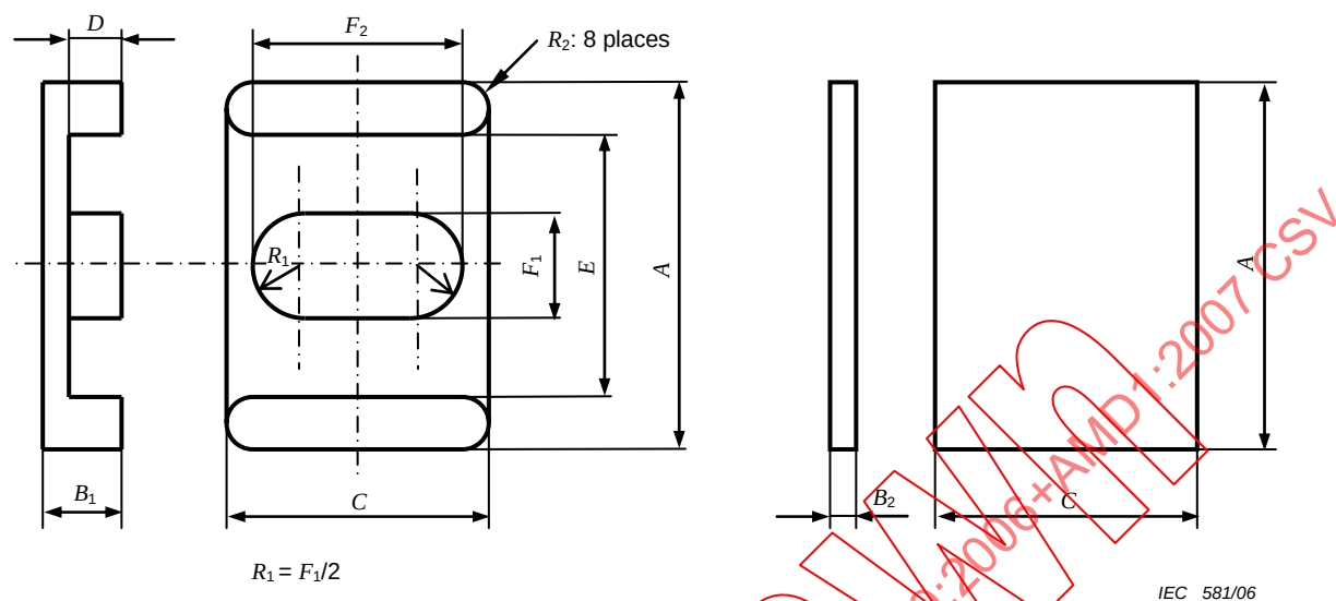
Figure 1 – Planar core EL and the mating PLT-core
