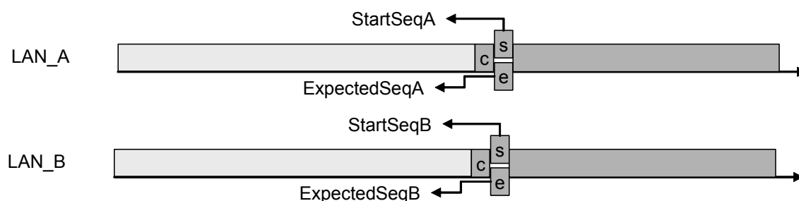
Figure 30 – PRP synchronized LANs
