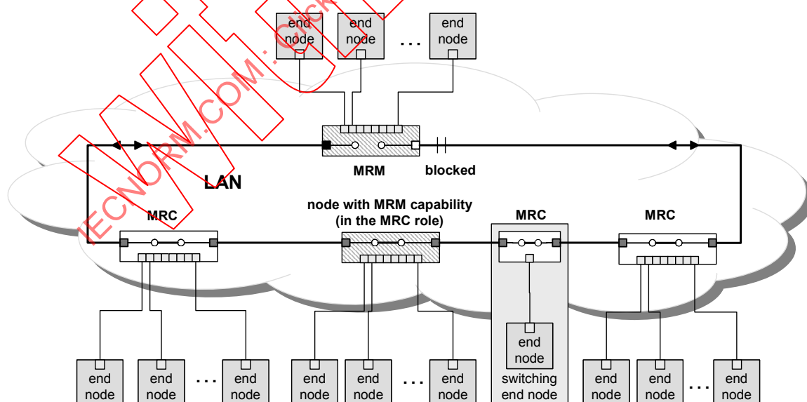
Figure 15 – MRP ring with more than one MRM
