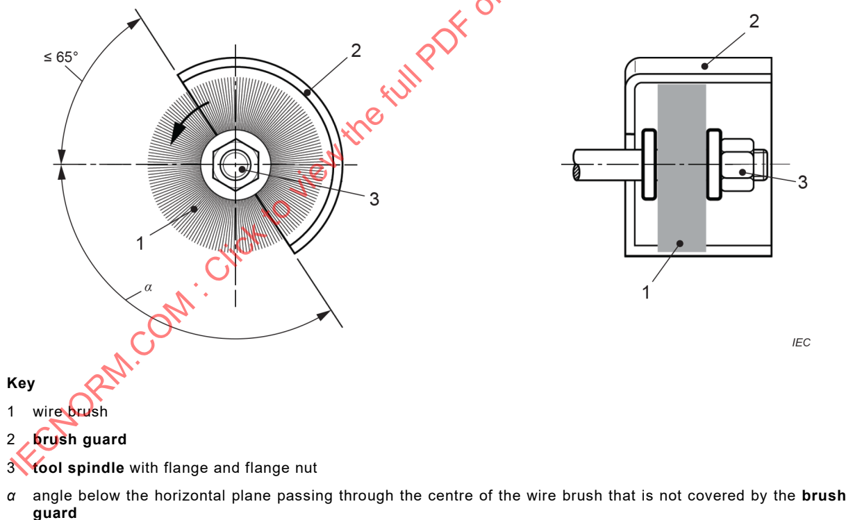
Figure 107 – Brush guard
