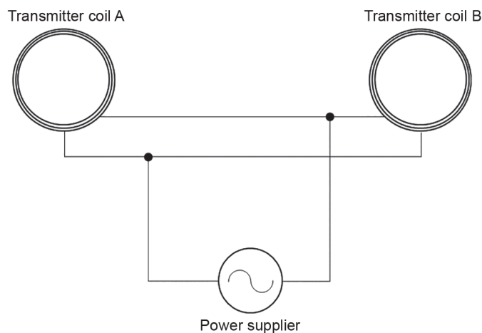
Figure 10 – Example of transmitter coils and a power supplier in an SWPT-MMR system
