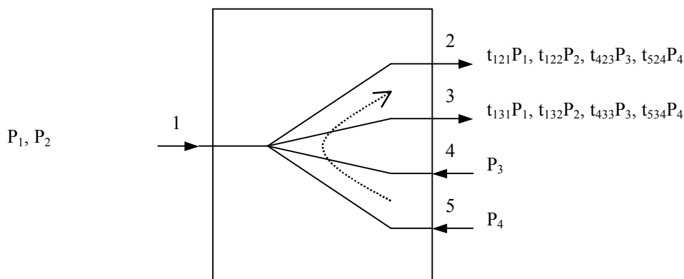
Figure 5 – Illustration of a four-wavelength bidirectional system
