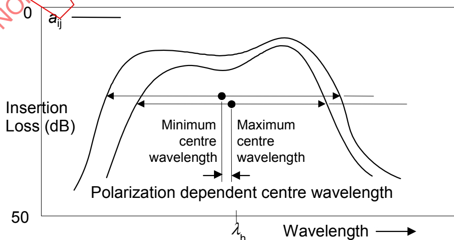
Figure 16 – Illustration of polarization dependent centre wavelength (PDCW)
