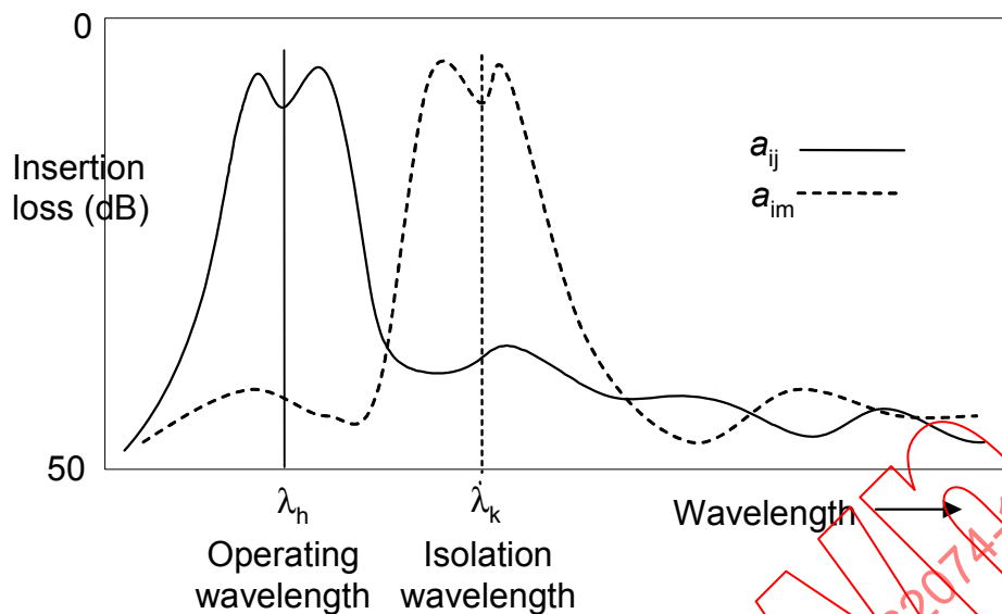
Figure 10 – Illustration of isolation wavelength
