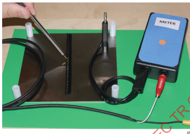
Figure 5 – Single point probe test method set-up
