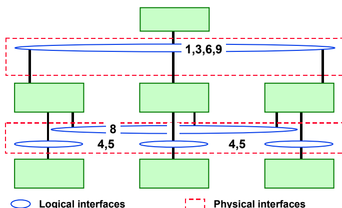
Figure 6 – Mapping of logical interfaces to physical interfaces; mapping of logical interface 8 to the process bus
