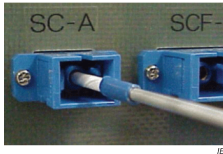
Figure 11 – Cleaning ports using a stick type cleaner
