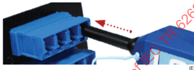
Figure 12 – Cleaning ports using a pen type cleaner
