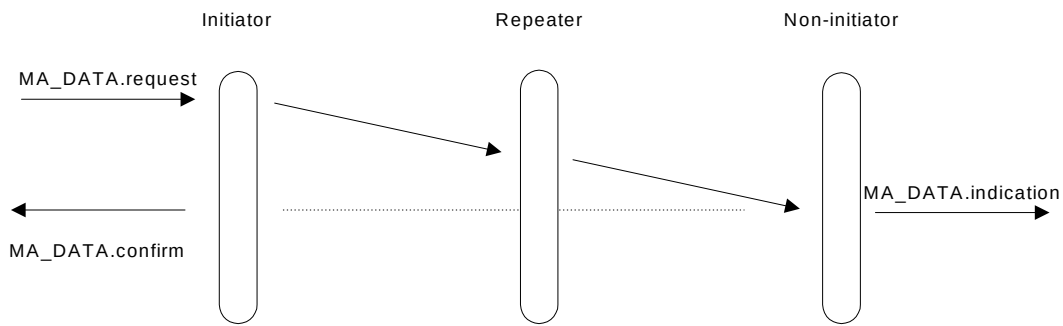
Figure 5 – MAC transmission using MAC service class 0 (postponed confirmation)
