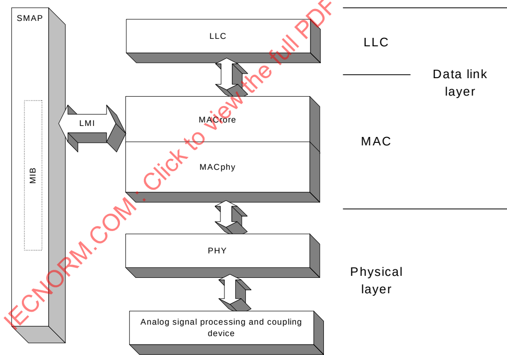
Figure 1 – Layered architecture of the DLC-M protocol stack
