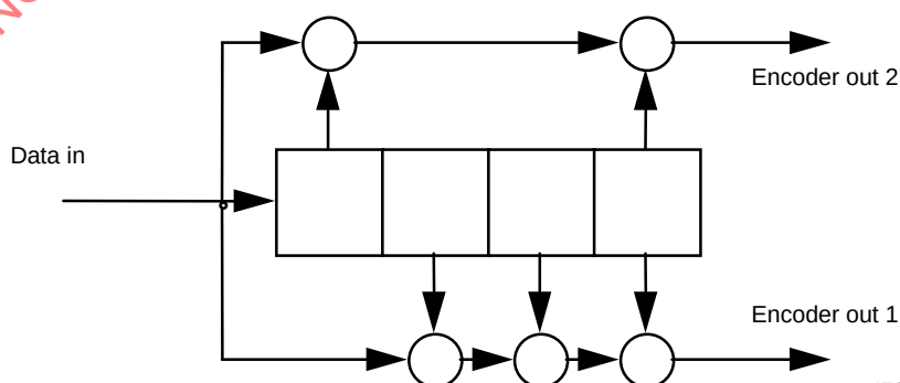
Figure 4 – Block diagram of encoder
