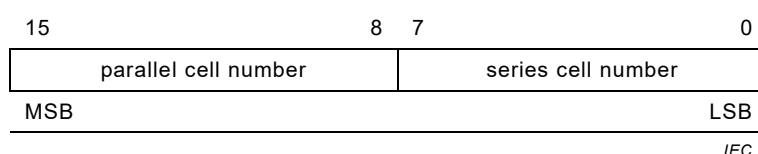
Figure 4 – Object structure
