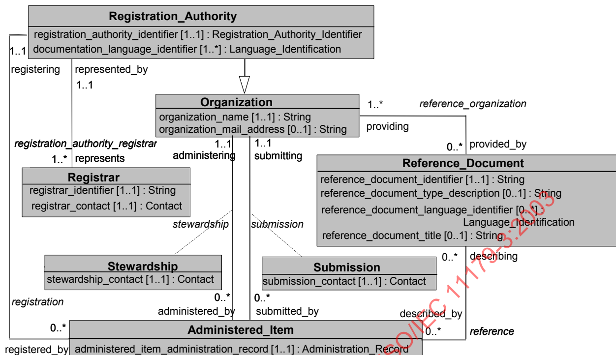
Figure 4 — Administration and identification metamodel region
