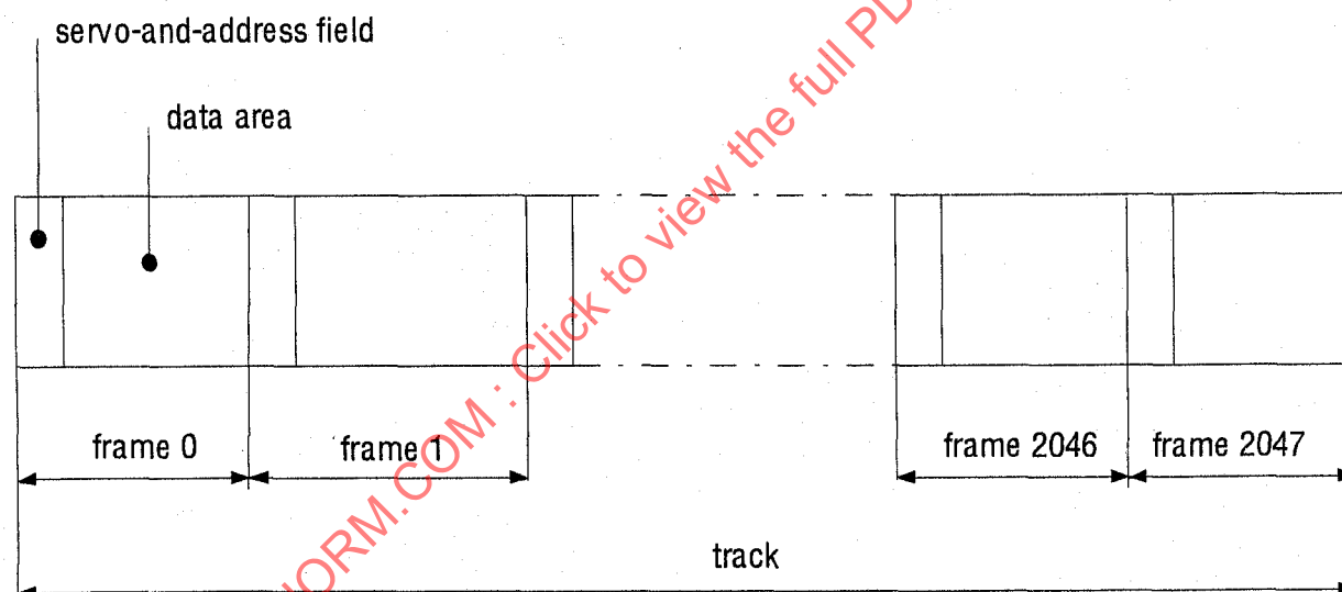
Figure 15 - Track layout
