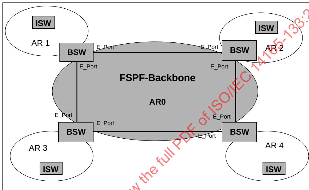
Figure 22 – FSPF-Backbone Architecture
