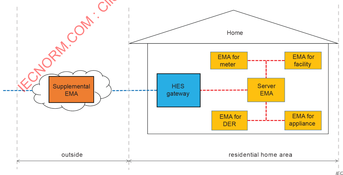
Figure A.3 – Hybrid EMA topology model example for a home
