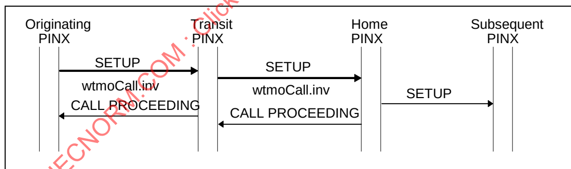
Figure C.7 - Successful invocation of ANF-WTMO with en-bloc operation
