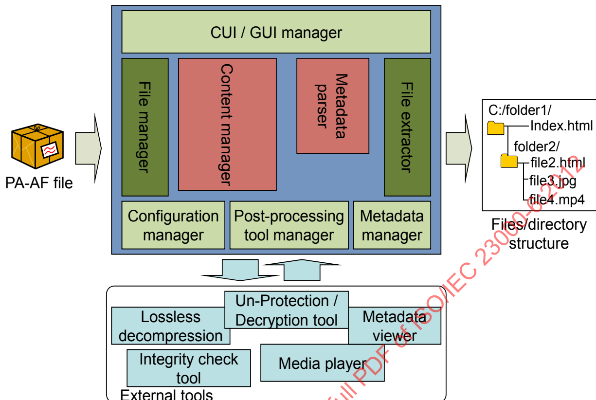
Figure 11 — PA-AF file extractor system architecture
