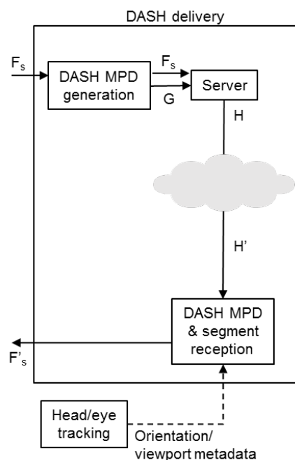
Figure 22 – Content flow in the DASH delivery function of OMAF
