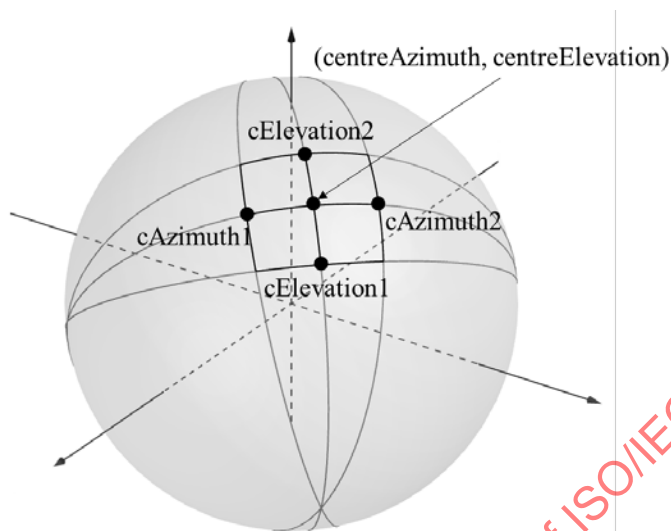
Figure 19 – A sphere region specified by four great circles
