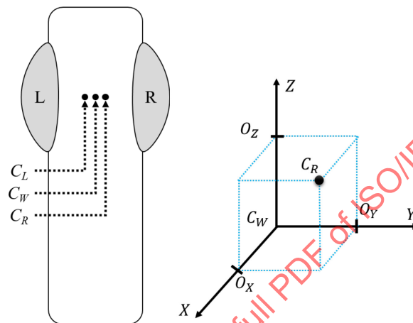
Figure 9 – Illustration of camera_centre_offset_x ( O_X ), camera_centre_offset_y ( O_Y ) and camera_centre_offset_z ( O_Z ) of the focal centre ( C_L or C_R ) of the fisheye camera lens (L or R, respectively) relative to the focal centre origin of the overall fisheye camera configuration ( C_W )
