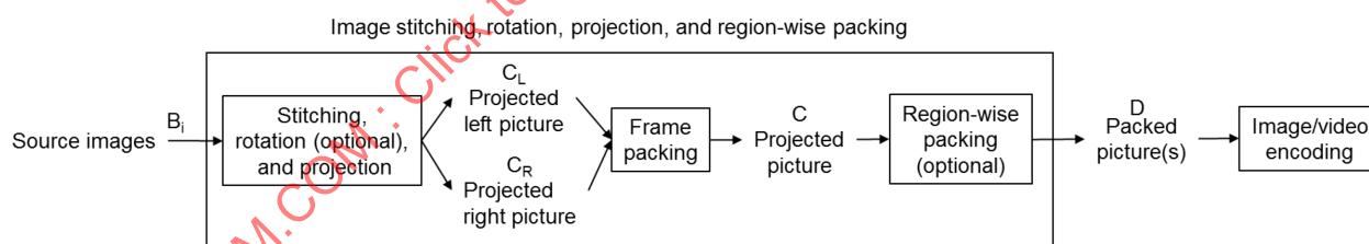
Figure 3 — Stereoscopic image stitching, rotation, projection, and region-wise packing of source images of a single acquisition time instance
