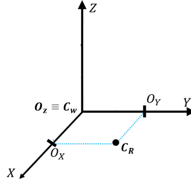
Figure 11 — Illustration of the entrance pupil rectification on the Z-axis
