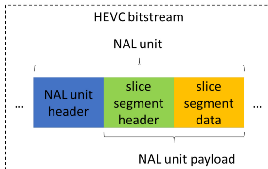
Figure 30 — Video data in HEVC bitstream
