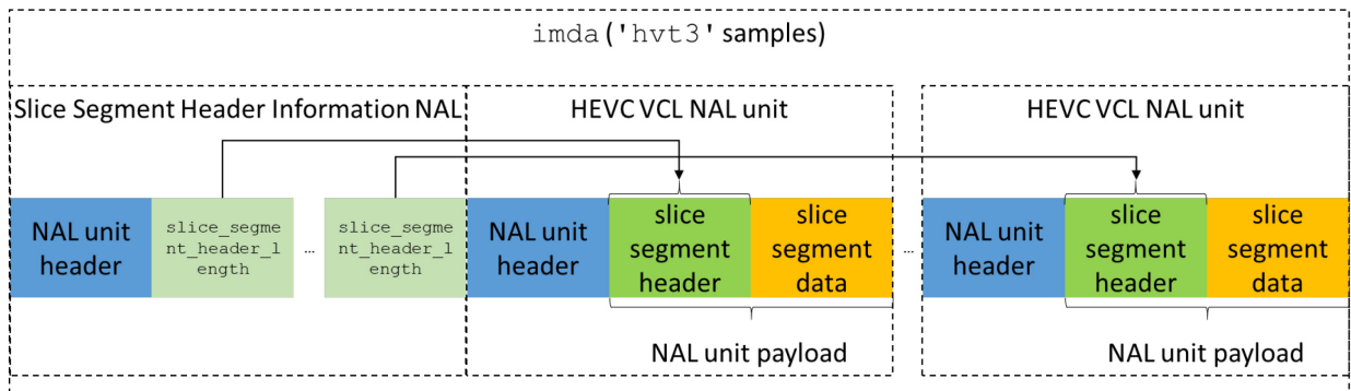
Figure 31 — Slice Segment Header Information NAL-unit-like structure in 'hvt3' tracks
