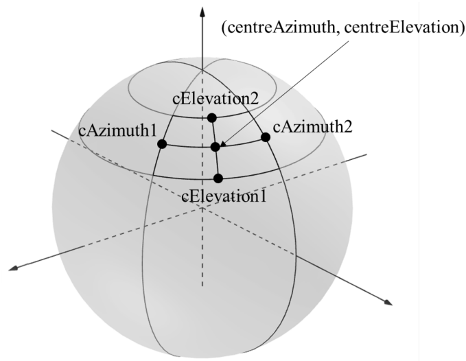
Figure 21 — A sphere region specified by two azimuth circles and two elevation circles
