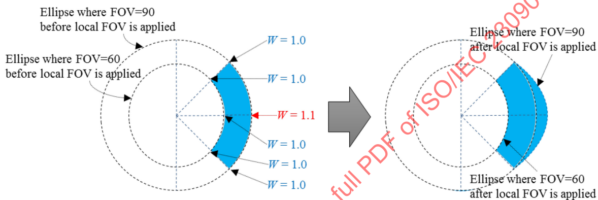
Figure 16 — Example of local FOV with a_s , a_e , and a_d equal to 45^\circ , 135^\circ , and 45^\circ , respectively, and r_s , r_e , and r_d equal to 0.5, 1.0, and 0.5, respectively
