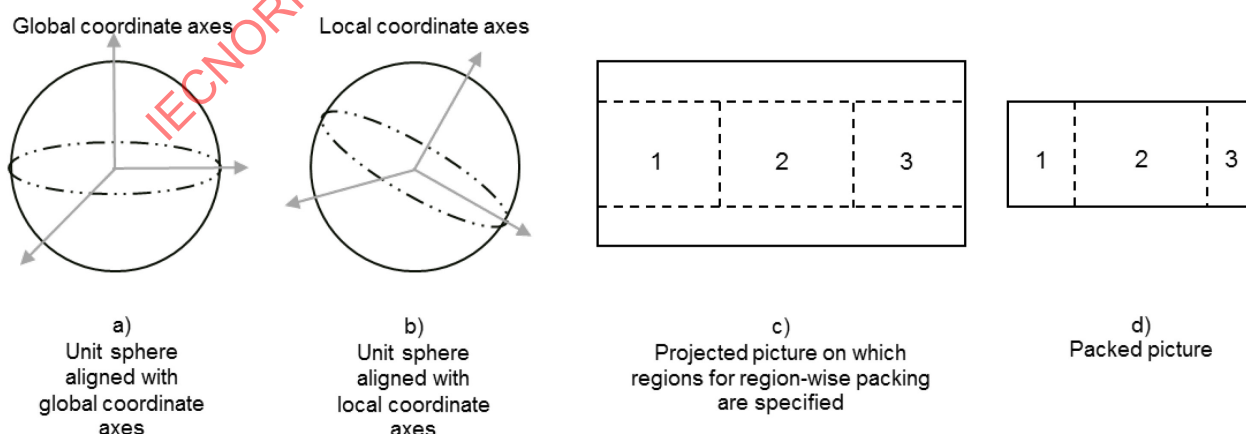
Figure 18 — Example of processing stages to derive a packed picture from a spherical image or vice versa
