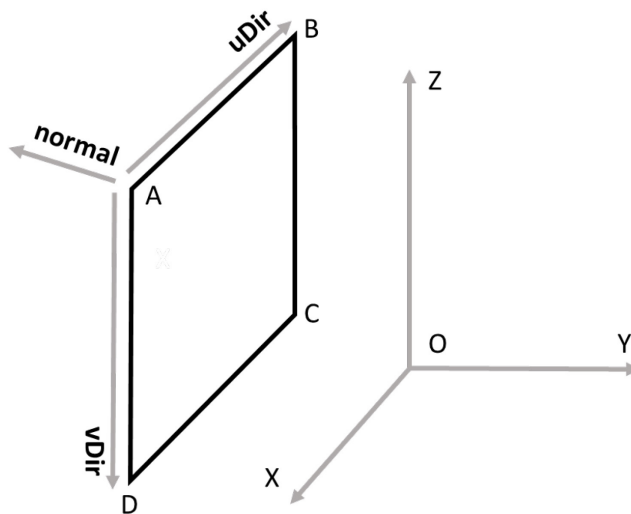
Figure 22 — 3D parallelogram
