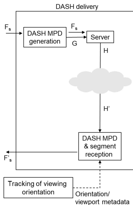
Figure 28 — Illustration of the content flow in the DASH delivery function of OMAF
