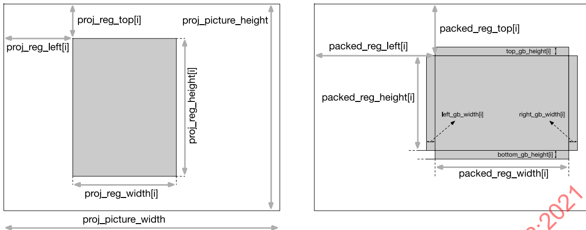
Figure 19 — An example of a projected region and the corresponding packed region with guard bands
