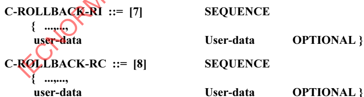
Figure 6 – C-ROLLBACK APDUs
