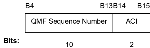
Figure 8-3a—Sequence Number field in QMFs
