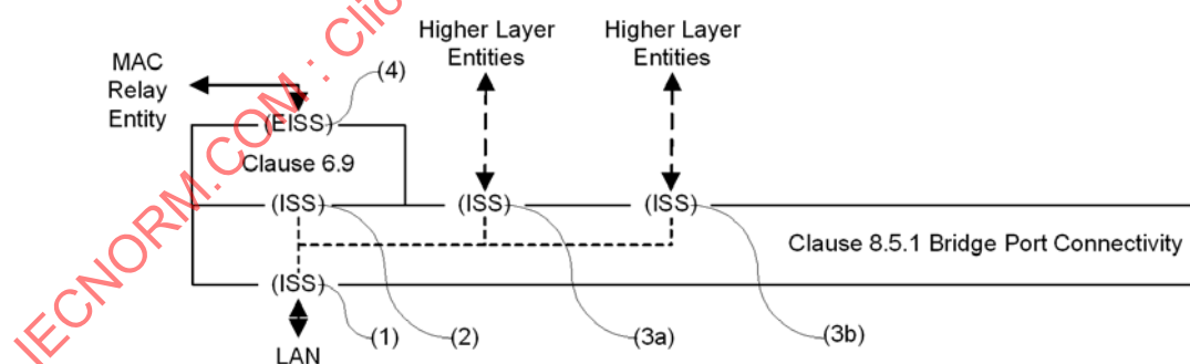
Figure 8-9—Bridge Port Transmit and Receive
