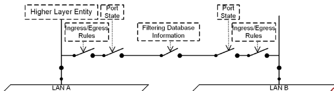
Figure 8-19—Ingress/egress control information in the forwarding path
