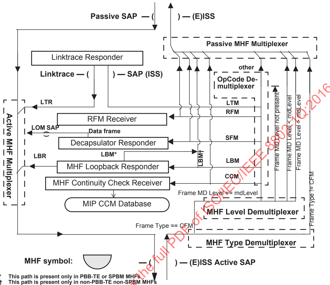
Figure 19-3—MIP Half Function (MHF)
