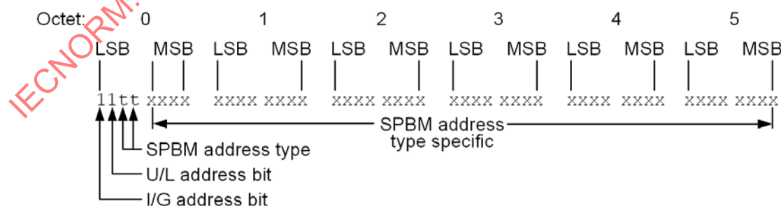
Figure 27-2—SPBM group MAC address—general format
