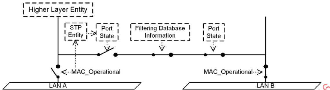
Figure 8-17—Effect of Port State
