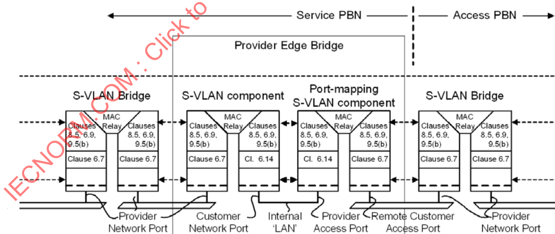
Figure 15-12—Port-based RCSI to a PBN
