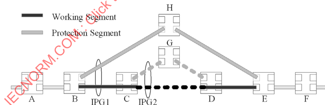
Figure 26-21—Nested IPGs
