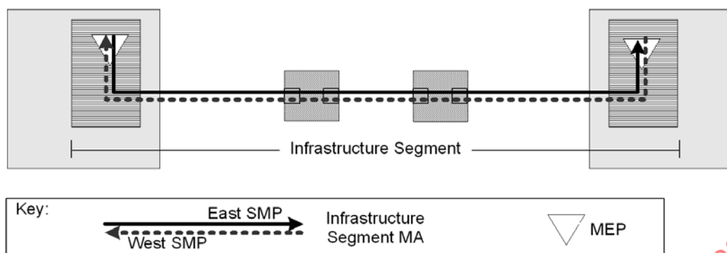
Figure 26-19—Infrastructure Segment monitoring
