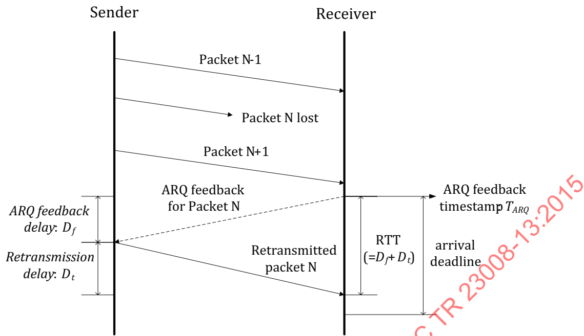
Figure 24 — Operation of the arrival-deadline constrained ARQ
