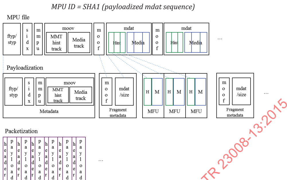
Figure 44 — Payloadized format
