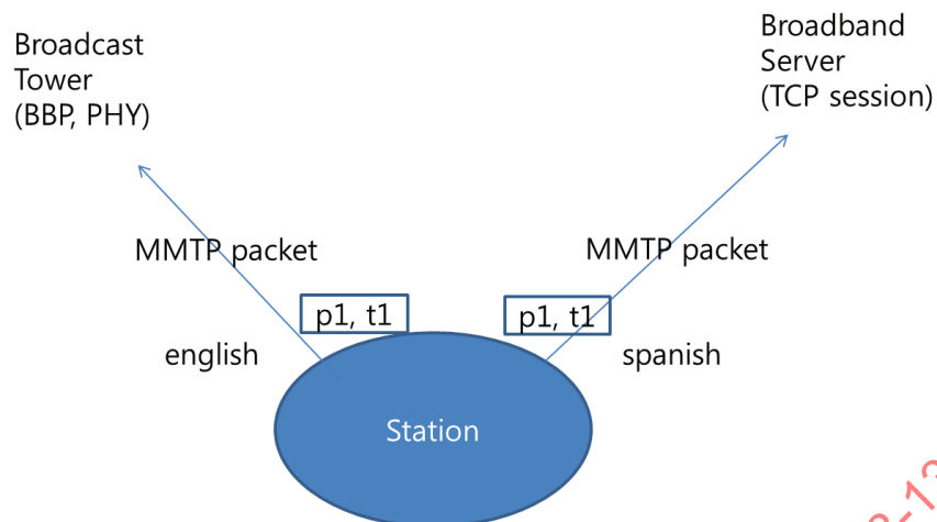
Figure 19 — Single station for hybrid delivery
