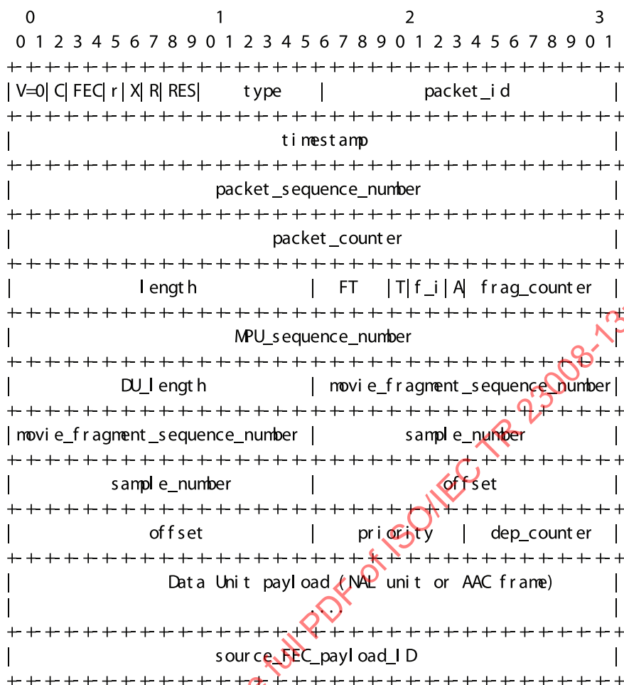
Figure 4 — MMTP packet
