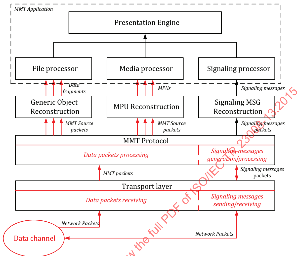
Figure 7 — MMT receiving entity structure
