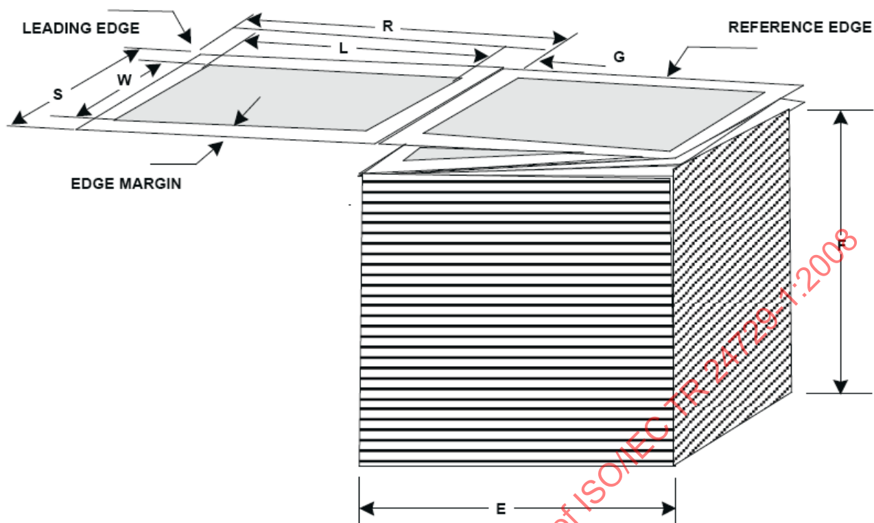
Figure A.2 – Label fanfold pack roll dimensions
