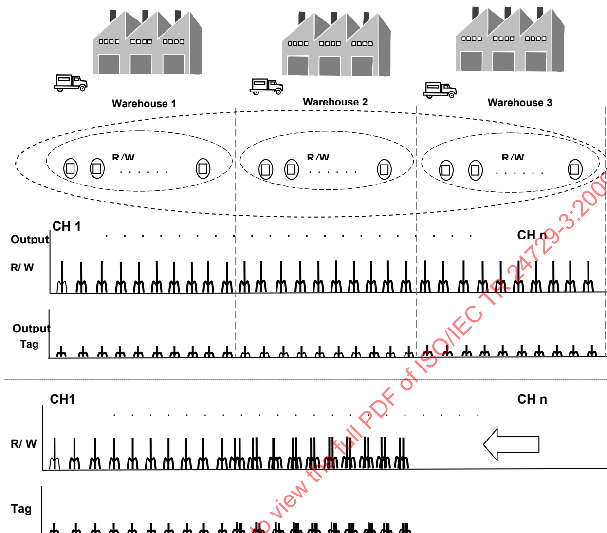
Figure 7 — Relationship between channel numbers and multi-interrogator system
