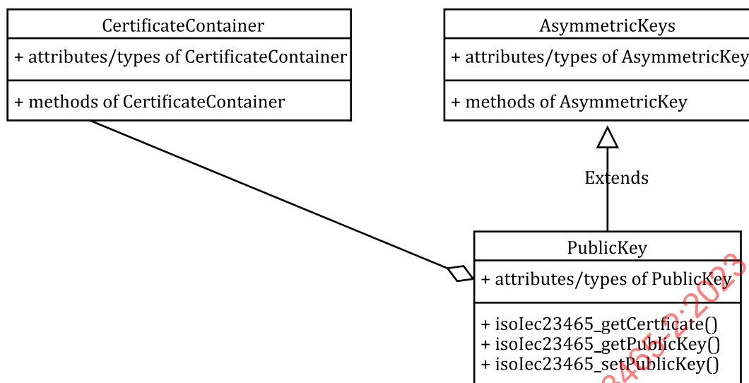
Figure 15 — PublicKey class
