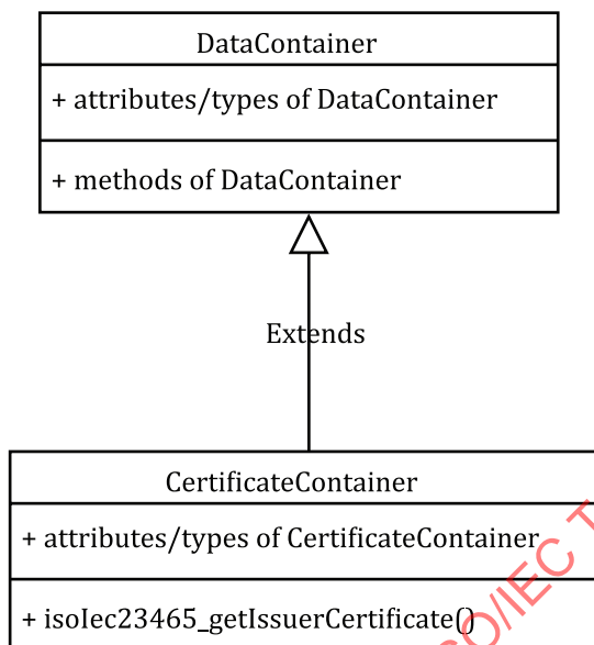
Figure 8 — CertificateContainer class
