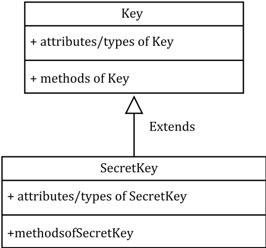
Figure 14 — SecretKey class
