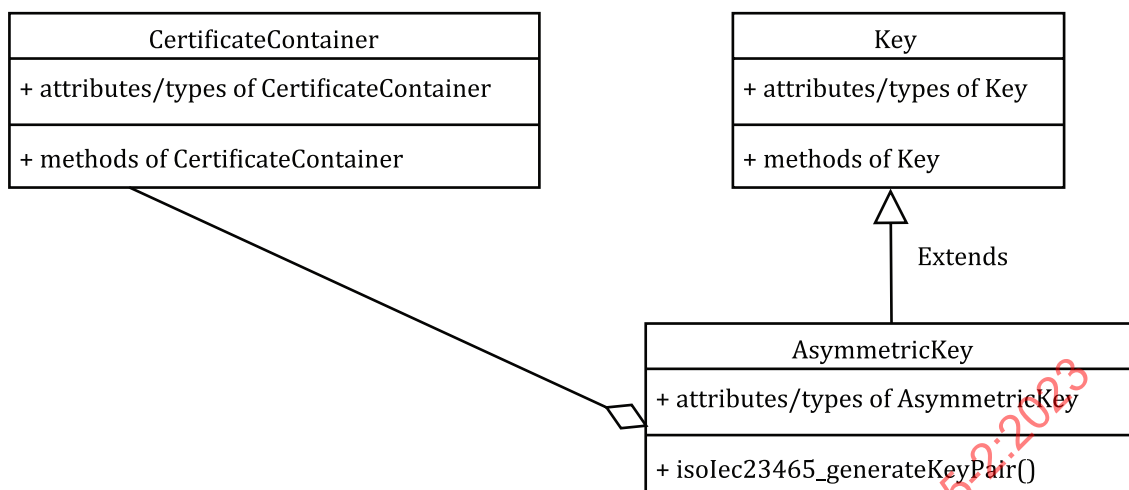
Figure 13 — AsymmetricKey class
