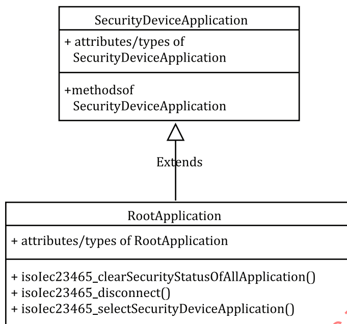
Figure 5 — RootApplication class
