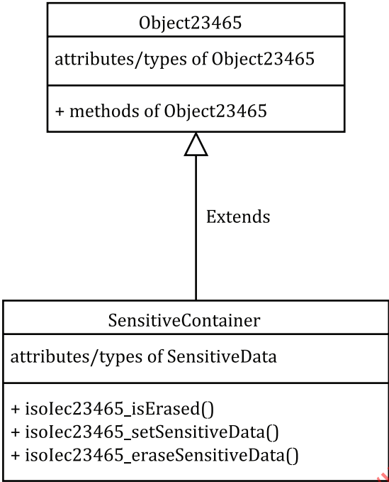
Figure 6 — SensitiveContainer class
