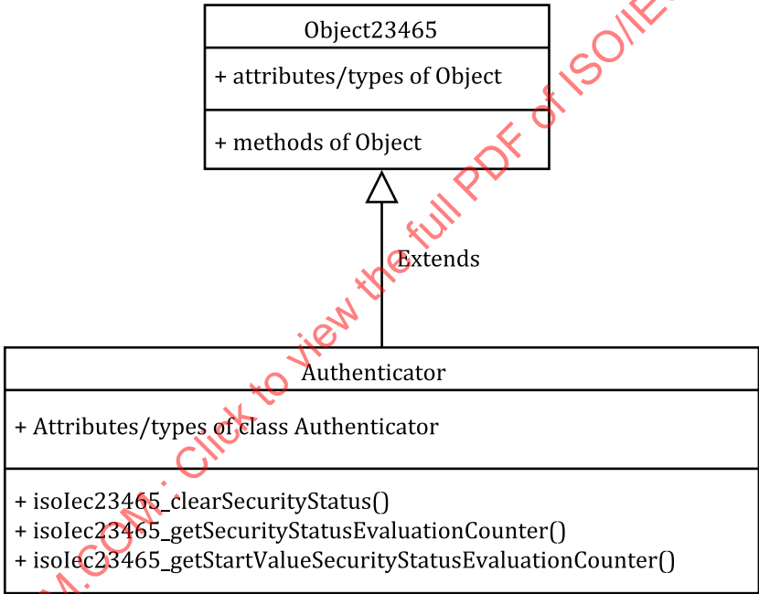
Figure 9 — Authenticator class
