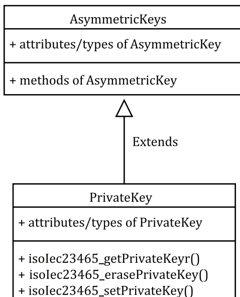
Figure 16 — PrivateKey class
