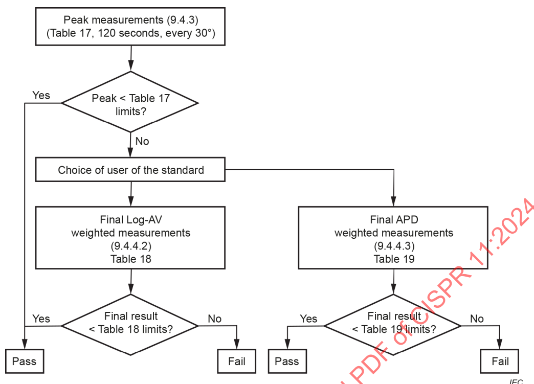
Figure 17 – Decision tree for the measurement of emissions from 1 GHz to 18 GHz of group 2 equipment operating at frequencies above 400 MHz
