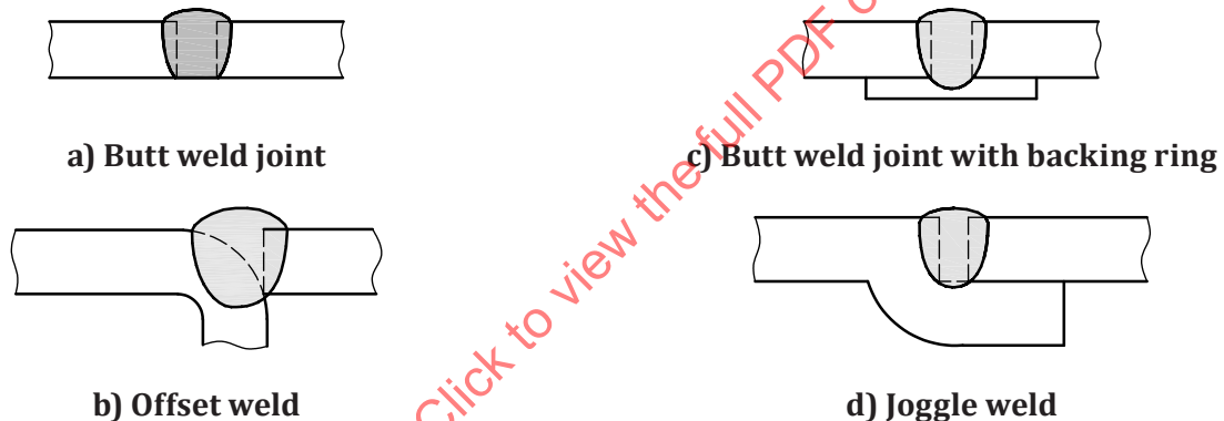
Figure 1 — Weld joints
