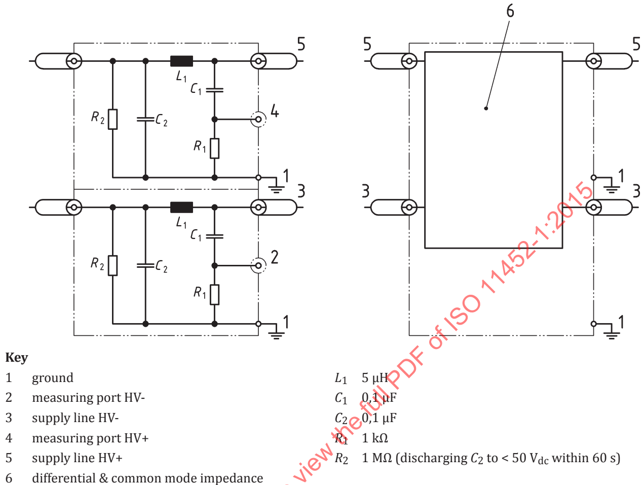
Figure B.6 — Impedance matching network attached between HV-ANs and DUT
