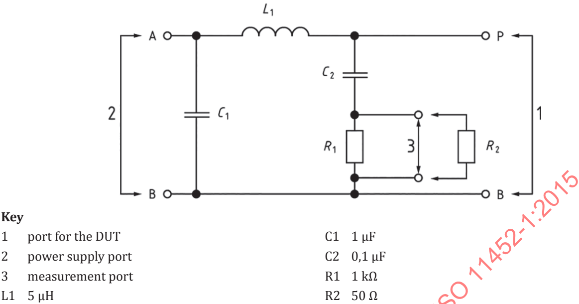
Figure B.1 — Example of 5 µH AN schematic
