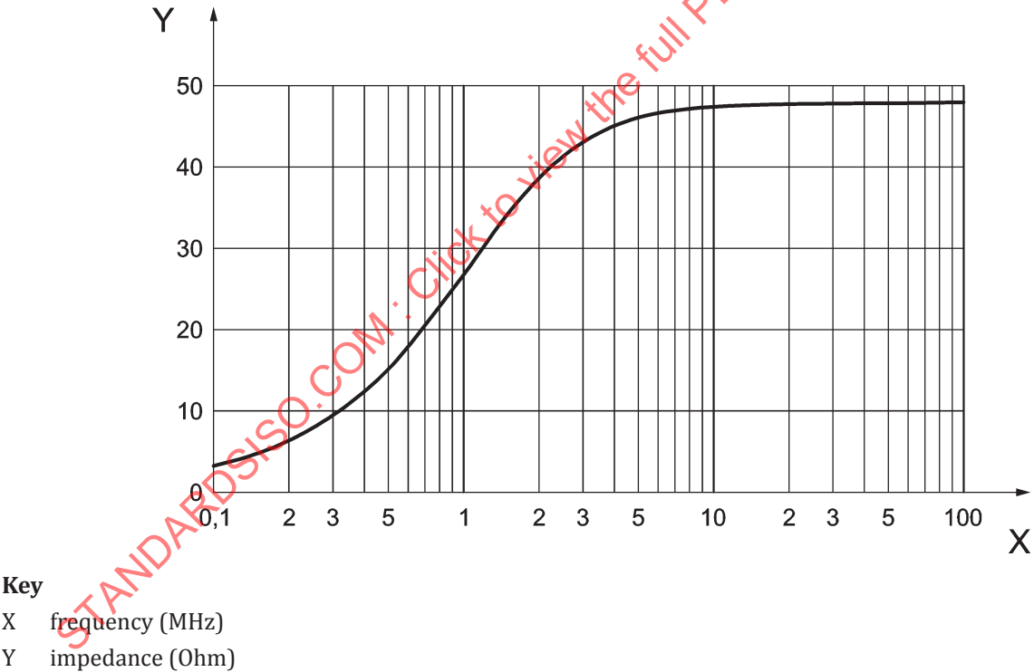
Figure B.2 — Characteristics of the AN impedance
