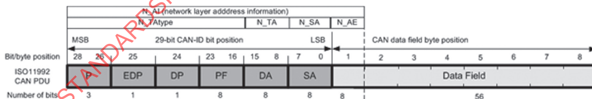
Figure 8 — Mixed addressing network layer address encoding (PDU1)
