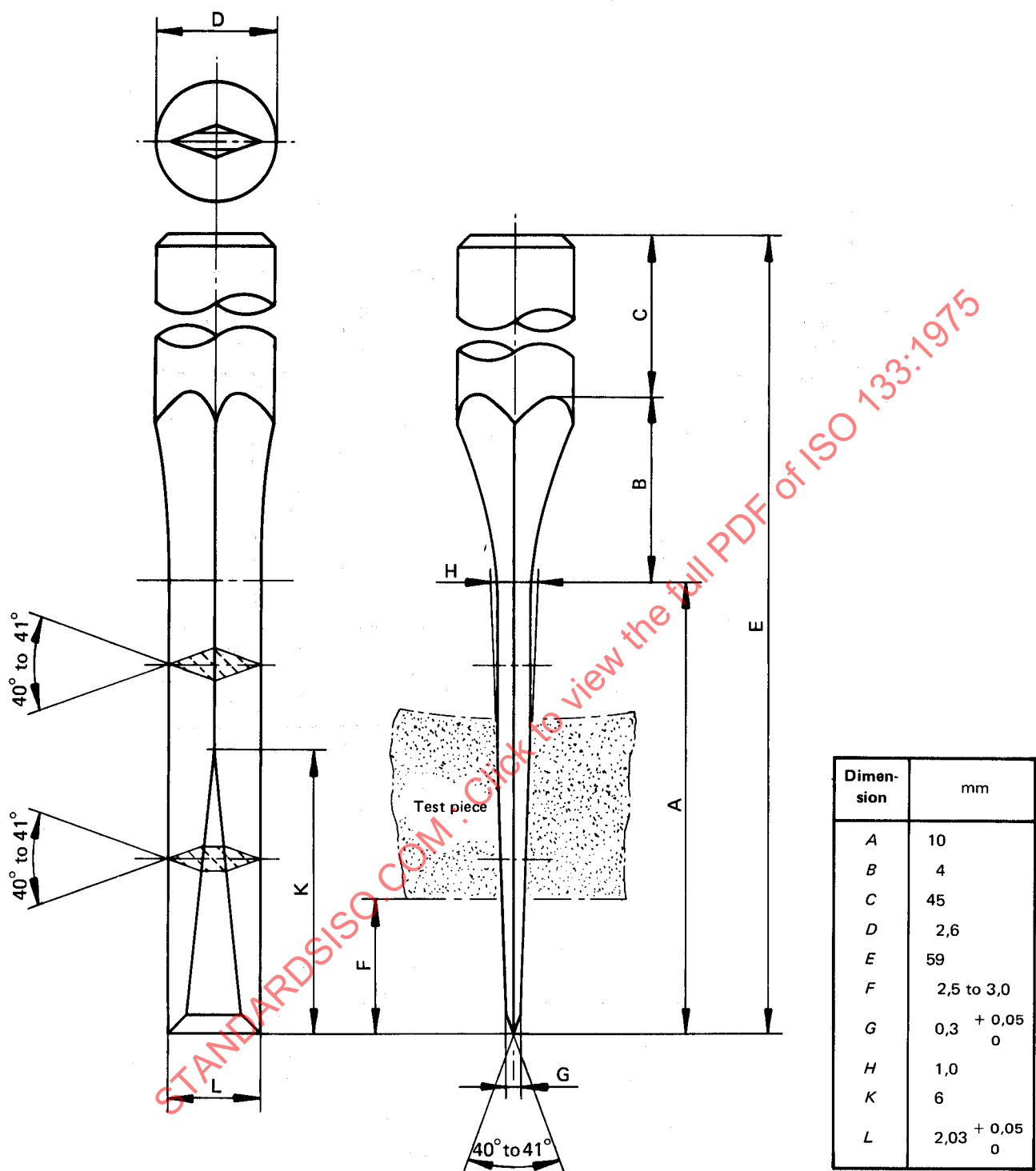
FIGURE 3 — Piercing tool
