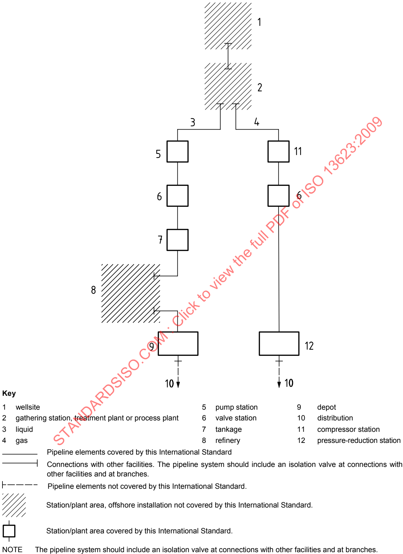
Figure 1 — Extent of pipeline systems covered by this International Standard
