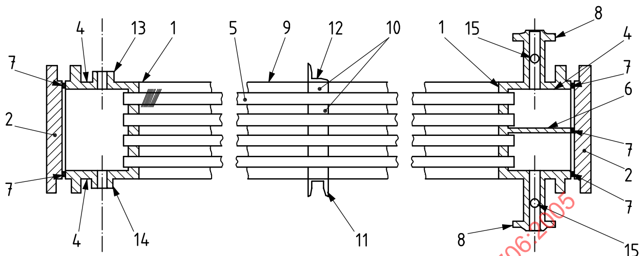
a) Removable cover-plate header
