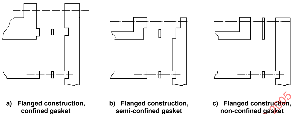
Figure 4 — Typical confined and full-faced gasket joint details
