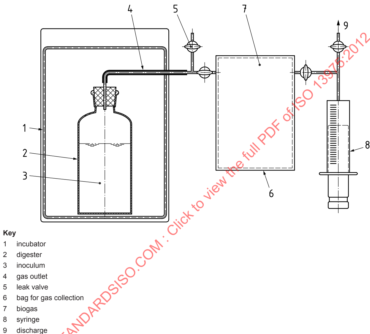
Figure A.1 — Example of a test system using a syringe to measure the volume of biogas produced
