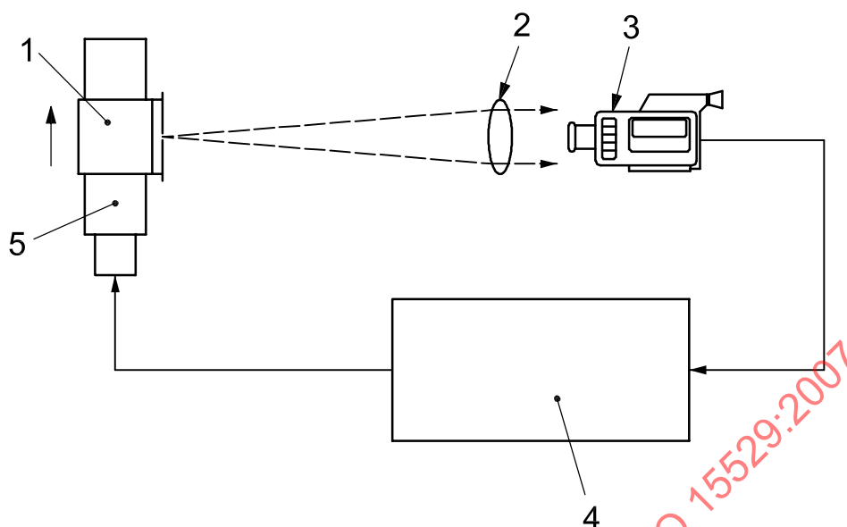
a) Schematic measurement arrangement
