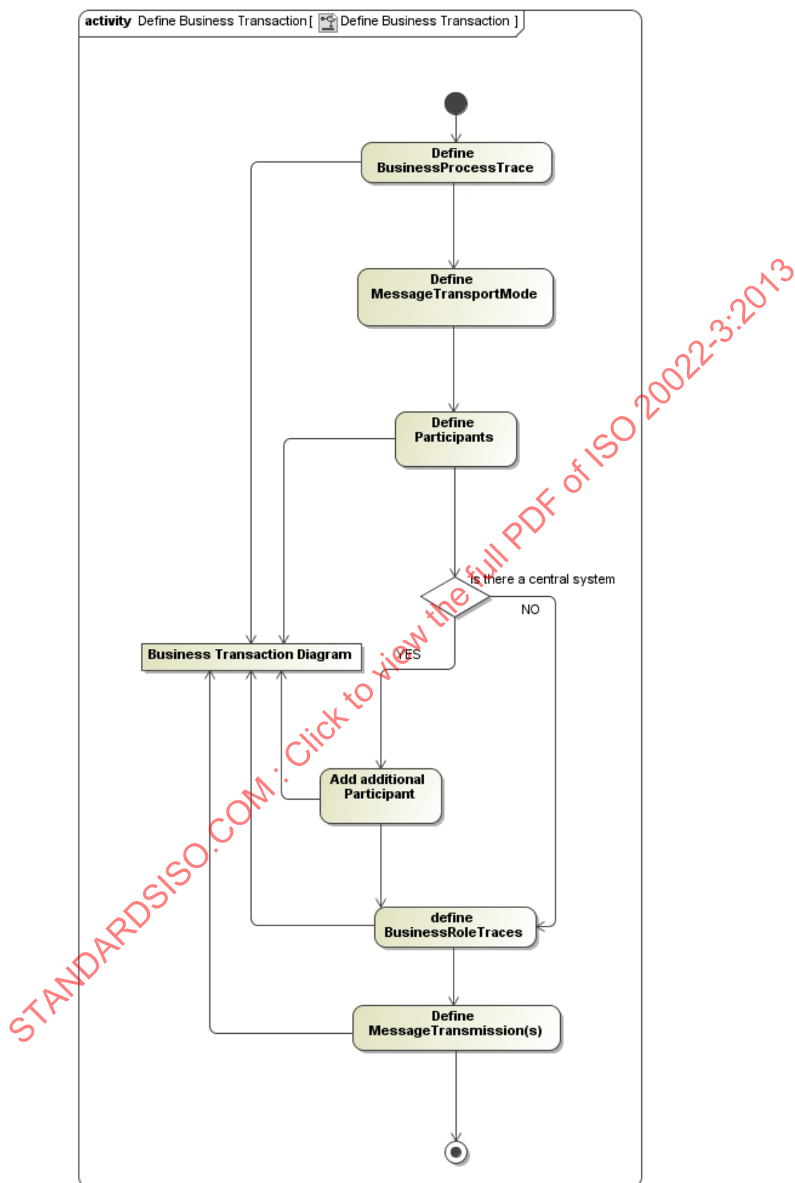
Figure 3 — Define BusinessTransaction
