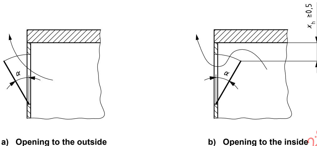
Figure B.2 — Examples of types of ventilator probably leading to negative discharge
