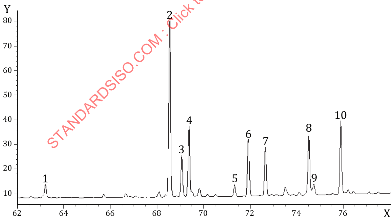
Figure A.1 — Typical chromatogram taken on an apolar column
