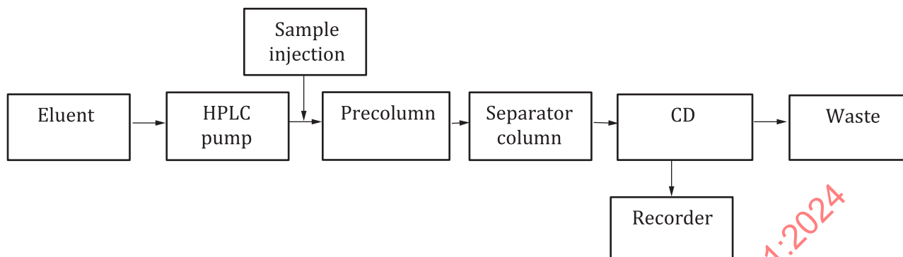
Figure 1 — Ion chromatography system
