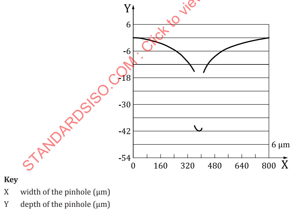
Figure A.10 — Pinhole — Profile
