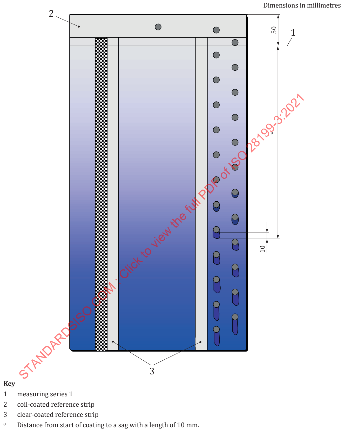
Figure 1 — Example for the assessment of the tendency to sagging
