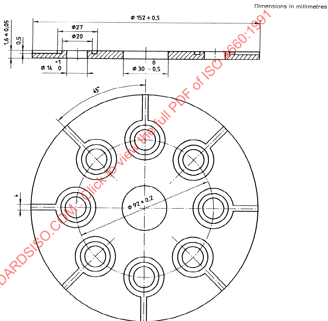
Figure 1 — Mould for colour index test
