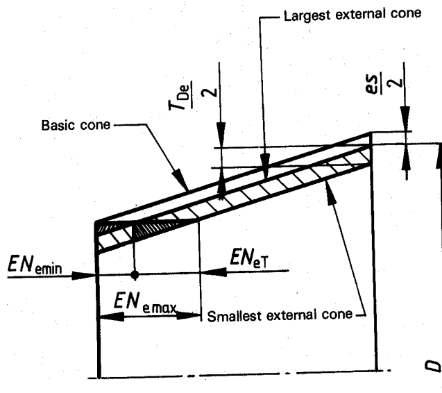
a) External cone — Positions of deviations a to g
