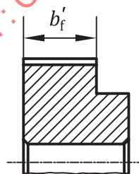
b) Unflanged pulley
