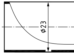
Figure 9 — External diameter indication
