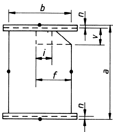
b) Internal sleeve valve
