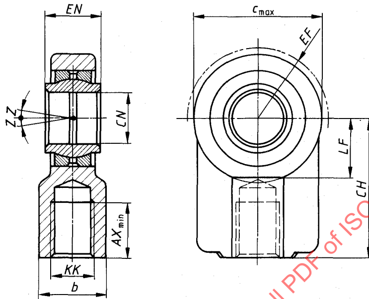
Figure — Rod end spherical eyes of hydraulic cylinder
