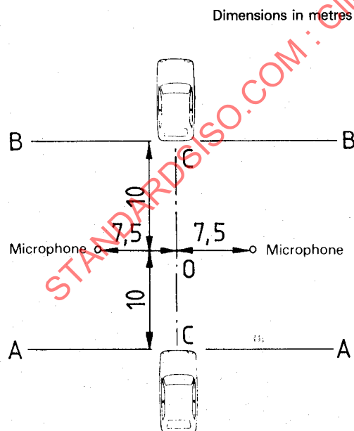
Figure 2 – Microphone positions for measurements
